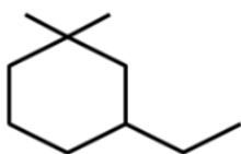
1-Ethyl-3,3-dimethyl cyclohexane
