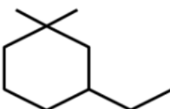
1-Ethyl-5,5-dimethyl cyclohexane
