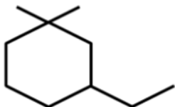
5-Ethyl-1,1-dimethyl cyclohexane
