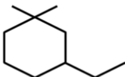
3-Ethyl-1,1-dimethyl cyclohexane
